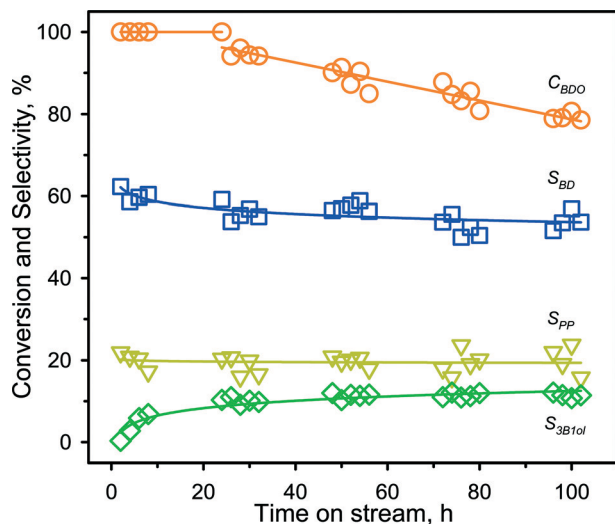
Fig. 2 Catalytic stability over ZSM-5@260 at 300 °C. Reaction conditions: T , 300 °C; ambient pressure, catalyst loading, 200 mg; liquid flowrate, 2.8 mL h -1 ; carrier gas flowrate, 60 mL (STP) min -1 . Nomenclature: C_{BD,0} , 1,3-BDO conversion; S_{BD} , selectivity to BD; S_{PP} , selectivity to PP; S_{3B1ol} , selectivity to 3-buten-1-ol.
