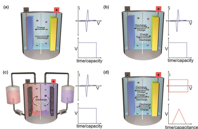
Fig. 1 Schematic depicting the working principle of (a) metal-ion batteries, (b) dual-ion batteries, (c) redox flow batteries, and (d) supercapacitors. The insets show the ideal electrochemical behaviour of each type of device when measured using cyclic voltammetry and galvanostatic charging/discharging. Here, V is voltage and i is current.
