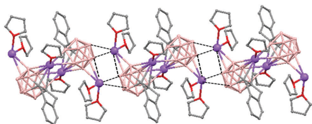
Fig. 12 1D-polymer chain of (69). H atoms omitted for clarity.
