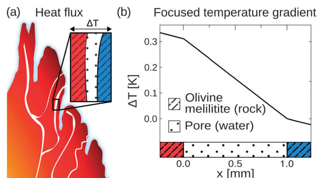
Fig. 2 Heat flux across porous rocks. (a) Formation of temperature gradients across porous rocks, heated by volcanic activity against the cold surrounding. Shallow temperature gradient settings can be found in various environments such as volcanic, water-vapour, or hydrothermal settings. (b) Simulations show that a difference in heat conductivity between the rock (olivine-melilitite \kappa = 2 \text{ W mK}^{-1} ) and the water filled pore ( \kappa = 0.6 \text{ W mK}^{-1} ) results in a local increase in temperature gradient across the pore by at least a factor of 3. Taking other naturally occurring minerals like quartz, peridotite, or pyrite-silica into account, the temperature gradient could further increase e.g. by a factor of 33 for the case of pyrite. Therefore, a minor temperature difference between both heat reservoirs suffices to enable highly efficient molecular accumulation.
