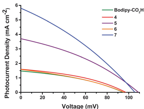
Fig. 3 Current-voltage characteristics of the dye-sensitized NiO solar cells with 0.1 M I _2 , 1.0 M LiI electrolyte and 4 (red), 5 (purple), 6 (orange), 7 (blue) and Bodipy-CO _2 H (green) under AM 1.5G (100 mW cm ^{-2} ) illumination.
