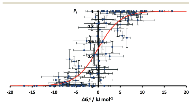
Fig. 4 Relationship between \Delta G_i^\circ and p_i for all functional group combinations in Table 1 (RMSE = 0.20). The red line corresponds to the Boltzmann distribution in eqn (5).
