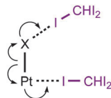
Chart 2 The Pt–X bond elongation caused by the \text{HI}_2\text{C}-\text{I}\cdots\text{X}-\text{Pt} and \text{HI}_2\text{C}-\text{I}\cdots\text{Pt} weak interactions.
