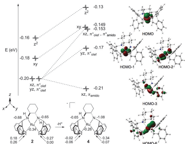
Fig. 2 Top left: Partial orbital energy diagram on going from 2 to 4 with relative orbital energies given in eV. Right: Kohn-Sham orbitals of 4 (isovalence = 0.06). Bottom left: Selected APT charges of 2 and 4 given in ESU.
