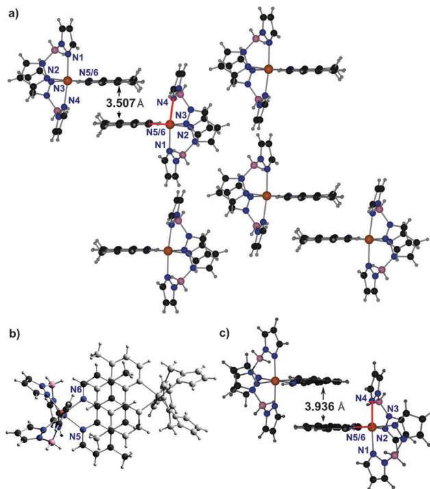
Fig. 2 1D stacking motifs in 6 ·0.5 \text{C}_7\text{H}_8 at 293 K in the side view (a) and in the top view (b). For comparison compound 2 (c) taken from Real et al. 4 Color code: C (black), H (grey), B (pink), N (blue), Fe (orange) and toluene (not shown).
