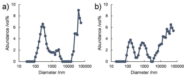
Fig. 3 Volume-based size distributions obtained by DLS for (a) 1 /[Co II -(MeO-terpy) 2 ] and (b) 2 /[Co II (MeO-terpy) 2 ] in water at 293 K. [Co] = 5 mM.
