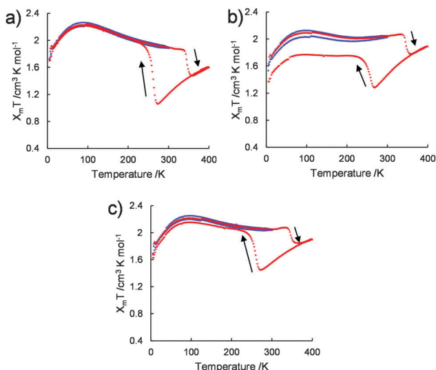
Fig. 4 \chi_{mT} versus T for (a) 1/[\text{Co}^{\text{II}}(\text{MeO-terpy})_2] , (b) 2/[\text{Co}^{\text{II}}(\text{MeO-terpy})_2] and (c) 3/[\text{Co}^{\text{II}}(\text{MeO-terpy})_2] on warming ( \blacktriangle ) and cooling ( \blacktriangledown ). The blue plots indicate the first cycle (from 5 to 300 K) and the red plots indicate the second cycle above the boiling point of water (from 5 to 400 K).
