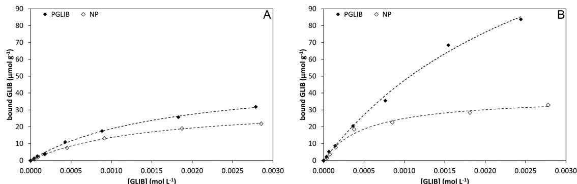
Fig. 5 Binding isotherms and corresponding Langmuir model fitted curves for P GLB and NP in acetonitrile (A) and chloroform (B).
