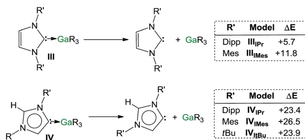
Fig. 7 Estimated dissociation energies ( \text{kcal mol}^{-1} ) of complexes III and IV ( \text{R} = \text{Dipp, Mes, I}^t\text{Bu} ).
