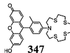
Fig. 307 Chemical structure of ligand 347 and its applications to detect Hg 2+ in live cells and in edible fish.
