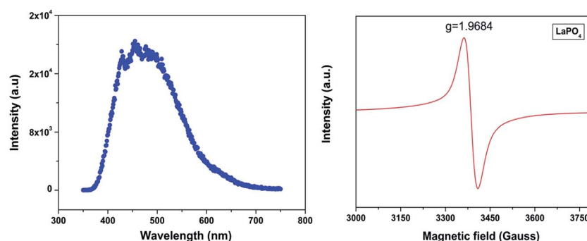
Fig. 4 (a) Emission spectrum of undoped \text{LaPO}_4 nanoparticles ( \lambda_{\text{ex}} = 230 \text{ nm} ) and (b) room-temperature EPR spectra of undoped \text{LaPO}_4 .
