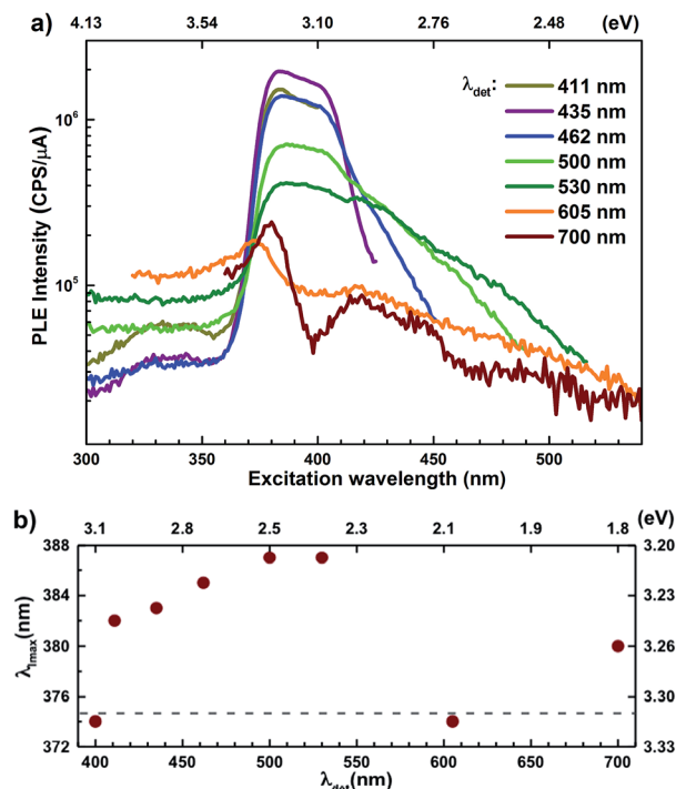
Fig. 5 (a) Semi-log plot of photoluminescence excitation spectra for different emission wavelengths for ZnO/ITO nanorods. (b) Position of maximum intensity peak ( \lambda_{lmax} ) for different detection wavelength.
