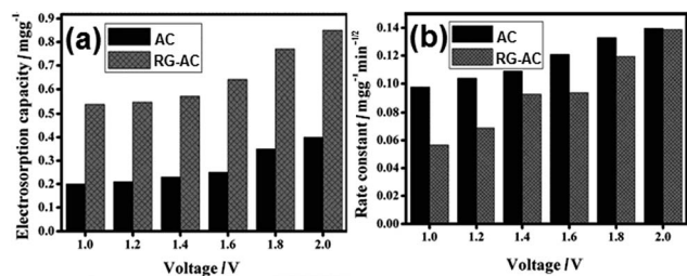
Fig. 8 (a) Electroadsorption capacity of the AC and RG-AC (20 wt% RG) electrodes at different voltages in NaCl solution with an initial conductivity of 50 \mu\text{S cm}^{-1} ; (b) rate constants of the electroadsorption kinetics for AC and RG-AC (20 wt% RG) electrodes at different voltages. (Reproduced with permission from ref. 90.)
