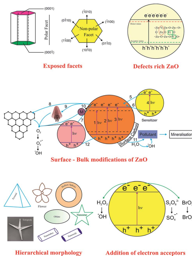
Fig. 30 Overall view of ZnO-based photocatalysis. The scheme at the four corners shows the reactive facets (top left), intrinsic defects (top right), nanostructured morphopology (bottom left) and the generation of free radicals with electron acceptors (bottom right). The centre image represents the charge transfer pathways in the surface-bulk modification of zinc oxide that are reported to improve the photoactivity. Path 1-excitation from VB to the dopant level (metal ions); Path 2-bandgap excitation of ZnO; Path 3: excitation from the impurity level (nitrogen or carbon doping) to CB; Path 4: excitation of the sensitizer (for instance, CdS, CuS, g-C 3 N 4 , inorganic complexes); Path 5: transfer of the excited electrons to the ZnO CB; Path 6: direct excitation of the electron from the sensitizer to the CB of ZnO (as observed in the surface complex formation between 4-CP and ZnO); Path 7 and 12: transfer of the electrons and holes in a bicomponent system (for instance ZnO-SnO 2 ); Path 8–10: electron trapping from graphene, MWCNTs and the metal islands on ZnO surface, respectively; Path 11: surface carbon enriches pollutant adsorption on the ZnO surface, thus facilitating the direct attack of the hole or the hole oxidizes water molecules to generate hydroxyl radicals.
