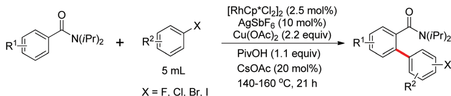
Scheme 60 Rh(III)-catalyzed dehydrogenative aryl–aryl bond formation.
