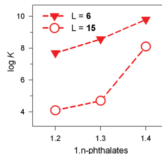
Fig. 27 Log K values for the equilibria: [\text{Cu}^{II}_2(\text{L})]^{4+} + \text{A}^{2-} \rightleftharpoons [\text{Cu}^{II}_2(\text{L})(\text{A})]^{2+} , where \text{A}^{2-} is a 1, n -phthalate: (i) filled triangles, \text{L} = \mathbf{6} , 50/50 (v/v) \text{H}_2\text{O} - \text{EtOH} , 25^\circ\text{C} . 39 (ii) empty circles, \text{L} = \mathbf{15} , water, 25^\circ\text{C} . 40
