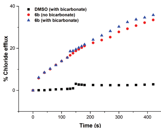
Fig. 6 Chloride efflux promoted by compound 6b (2% molar carrier to lipid) from unilamellar POPC vesicles loaded with 450 mM NaCl buffered to pH 7.2 with 20 mM sodium phosphate salts. The vesicles were dispersed in 162 mM \text{Na}_2\text{SO}_4 buffered to pH 7.2 with 20 mM sodium phosphate salts. At t = 120 s, a solution of \text{NaHCO}_3 was added to give a 40 mM external concentration (blue markers) or the experiment was allowed to continue without the addition of \text{NaHCO}_3 (red markers). At the end of the experiment, detergent was added to lyse the vesicles and calibrate the ISE to 100% chloride efflux. Each point represents the average of three trials.
