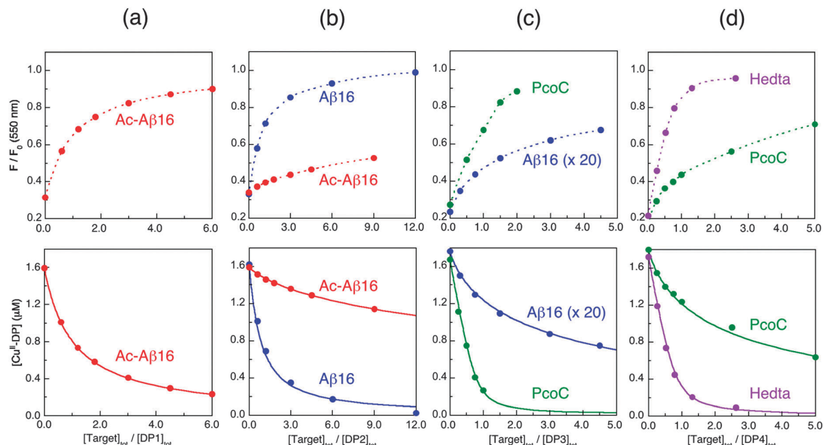
Fig. 10 Determination of conditional K_D for various protein/peptide targets in MOPS buffer (50 mM, pH 7.4): (a) Ac-Aβ16 with DP1 probe; (b) Ac-Aβ16 and Aβ16 with DP2 probe; (c) Aβ16 (note: 20× conc.) and PcoC with DP3 probe; (d) PcoC and Hedta with DP4 probe. Top panel showed recovering of the DP fluorescence intensity upon titration of each \text{Cu}^{\text{II}}\text{-DP} complex ( x = 0.8\text{--}0.9 ) with related competing Target ligands where the dot traces are the simple interpolations of the experimental points, and bottom panel gave correlation of [\text{Cu}^{\text{II}}\text{-DP}] versus [\text{target}]_{\text{tot}}/[\text{DP}]_{\text{tot}} where the solid traces are the fitting curves of the experimental data to eqn (11) that allowed determination of conditional K_D for each peptide/protein target as given in Table 3.
