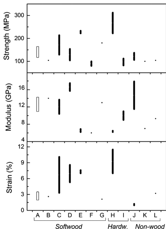
Fig. 6 Range of values for tensile properties of nanopapers investigated (A) compared with those reported in the literature from different sources of fibers (B–L). Softwoods: nanopapers from SEW fibers from Norway spruce of varying lignin content (present work) correspond to group A; B 30,31 (sulfite); C 32 (dissolving grade fibers); D 33 (bleached sulfite); E 34 (dissolving grade and bleached sulfite fibers); F 35 (bleached kraft); G 36 (bleached spruce sulfite). Hardwoods: H 37 (bleached kraft pulp); I 11 (birch kraft pulp). Non-wood: J 38 (swede root pulp); K 39 (sugar beet pulp chips); L 10 (palm fruit bunch fibers).
