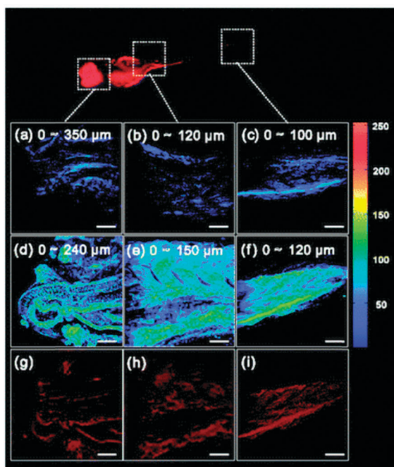
Fig. 15 Top: structure and reaction of aminonaphthalene probe P1 with \text{F}^- to form extended coumarin 20 . Bottom: accumulated TPM images for three zebrafish parts: (a–c) probe P1 alone (d–f) probe P1 followed by \text{F}^- (a–f) intensity data; (g–i) fluorescence images constructed by image stacking for 0–350 \mu\text{m} depth, with a 2 \mu\text{m} imaging depth step. Scale = 50 \mu\text{m} . View area: 300 \mu\text{m}^2 . Image reproduced with permission. 126
