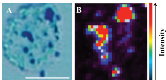
Fig. 2 Fixed MCF-7 cells on MIRR IR Low-E glass slides with 150 nm gold nanoparticles subsequently added. A light micrograph image in (A) shows labelling of MCF-7 cells with 150 nm nanoparticles (dark regions), which co-localize with areas of high Raman signal intensity in (B) (red areas). Scale bar = 10\text{ }\mu\text{m} .
