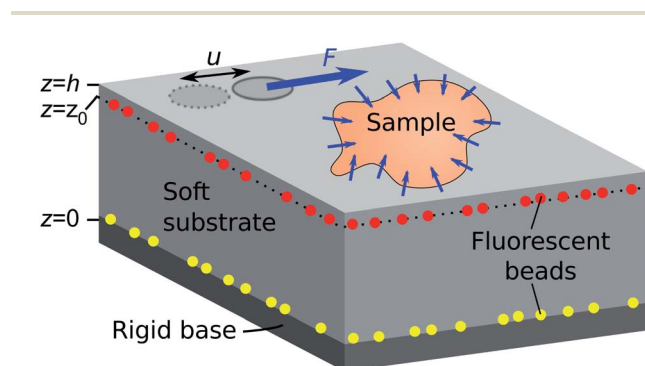
Fig. 5 Schematic diagram of a TFM substrate. A soft substrate (light grey) is bonded to a rigid base (dark grey). Fluorescent beads (yellow, red) are embedded at the substrate base, and near its surface. A discrete force, F , is applied to a finite patch (dark grey circle) of the substrate displacing it a distance u . A continuous stress distribution is applied by a contractile sample.
