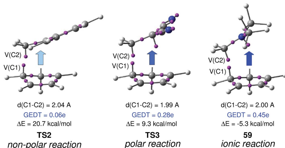
Fig. 16 Most relevant data of pseudodiradical structures involved in the C–C bond formation in the N-DA reaction of Cp 4 with styrene 5 , in the P-DA reaction of Cp 4 with DCE 6 , and in the I-DA reaction of Cp 4 with iminium cation 7 . The blue arrow indicates the direction of GEDT.
