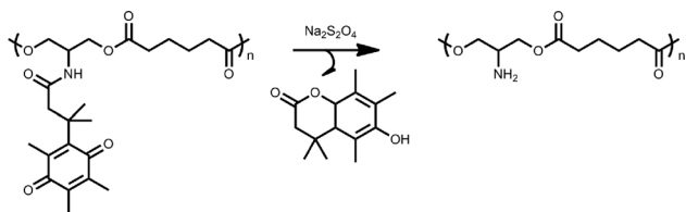
Scheme 10 TMPO shed from the polymer backbone upon reaction with sodium dithionite. 82
