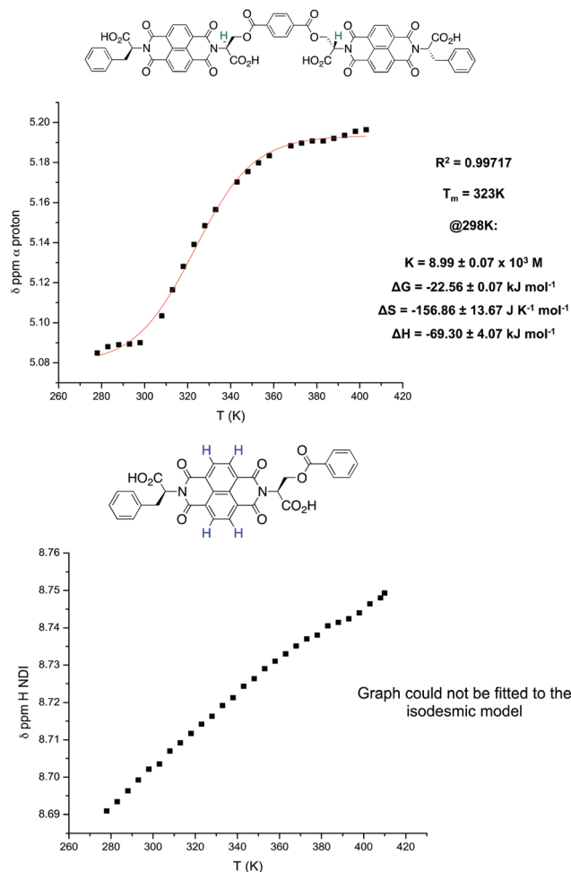
Fig. 7 Top: the isodesmic fitting and thermodynamic functions for the \alpha proton of 2 in 2% THF in TCE at 5 \times 10^{-4} M. Bottom: the loss of sigmoidal character for 1 in the same solvent system at 1 \times 10^{-3} M.
