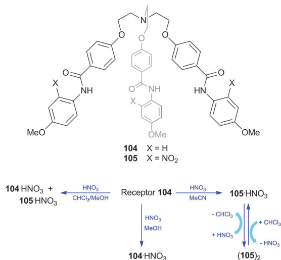
Scheme 12 Structure of receptor 104 and the nitro analogue 105 produced upon addition of \text{HNO}_3 , along with the various solvent-dependent conversions between receptor and complexes and dimers.
