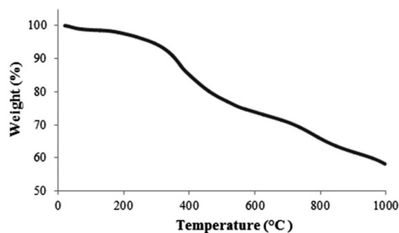
Fig. 4 TGA curve of MNPs 7 .
