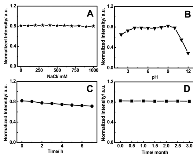
Fig. 4 (A) The relative fluorescence intensity at 427\text{ nm} (excitation at 344\text{ nm} ) of the FNCsPs in the NaCl solution. (B) Dependence of the fluorescence intensity on the pH values from 2 to 12. (C) The variation of the fluorescence intensity of the FNCsPs under irradiation by a 500\text{ W} Xe lamp for different time intervals. (D) Photostability of the FNCsPs as a function of the storage time.
