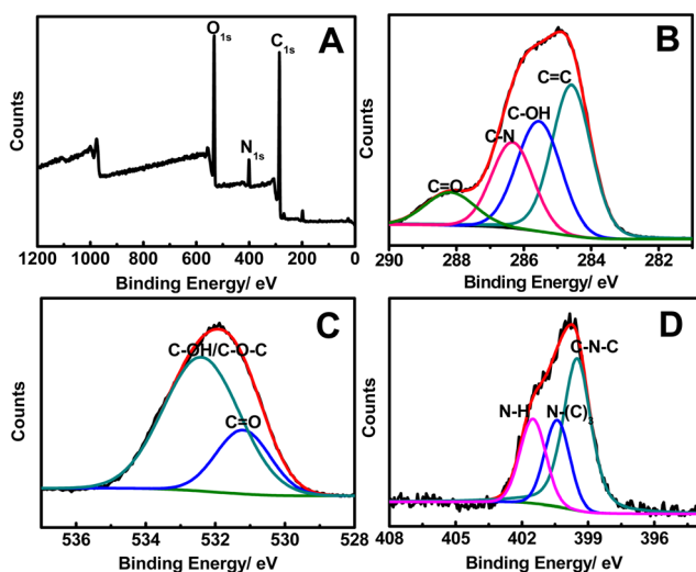
Fig. 3 The XPS (A), \text{C}_{1s} (B), \text{O}_{1s} (C), and \text{N}_{1s} (D) spectra of the as-obtained FNCsPs.
