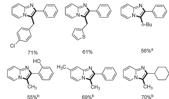
Scheme 62 Three-component reaction for the synthesis of imidazo[1,2-a]pyridines. a 2-Pentynoic acid was used; b propionic acid was used.
