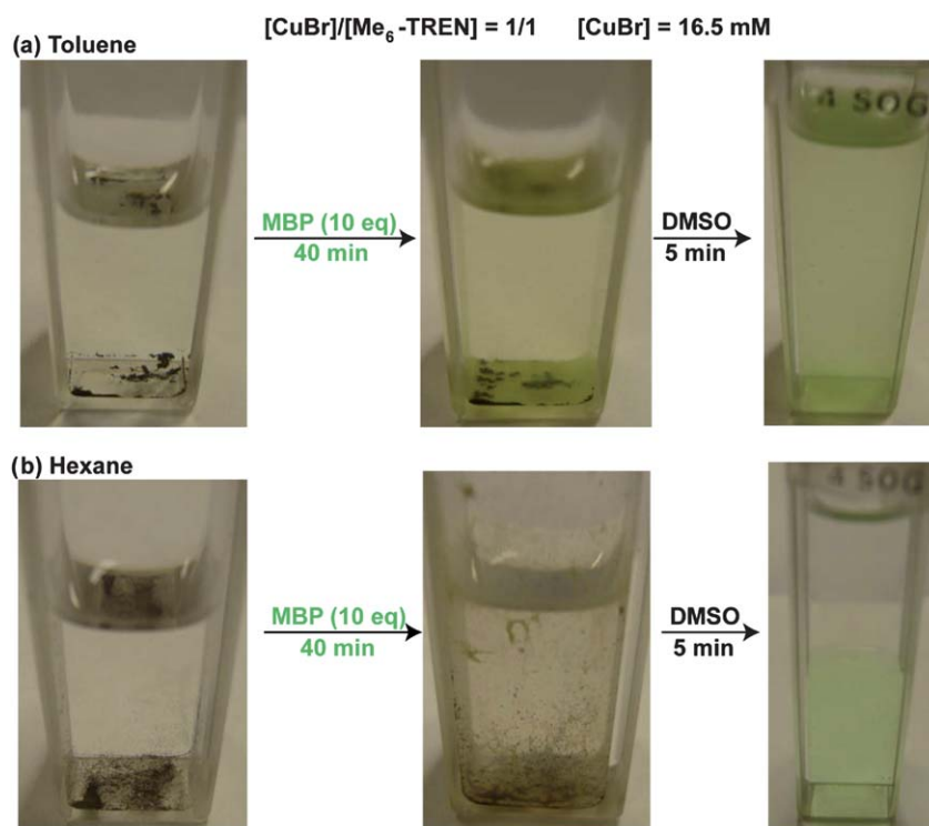
Fig. 11 Visual observation of Cu(0) nanoparticles and CuBr 2 generated from the disproportionation of CuBr in toluene (a); and hexane (b) before and after reaction the with MBP at 25 °C. MBP was added to the disproportionation mixtures after 40 min, followed by addition of 1.8 mL of DMSO. Conditions: solvent = 1.8 mL, [CuBr] = 16.5 mM, [MBP]/[CuBr]/[Me 6 -TREN] = 10/1/1.
