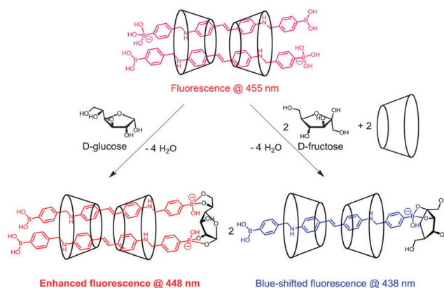
Scheme 5 Interaction of 2:2 35 -γ-CyD complex with D-glucose and D-fructose.
