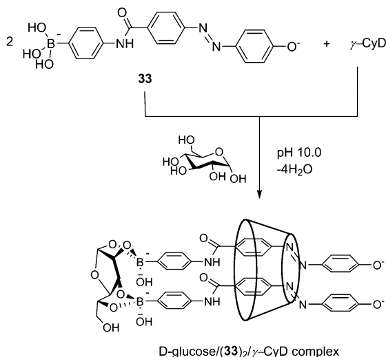
Scheme 4 2:1 inclusion complex of 33 with γ-CD in the presence of D-glucose. Adapted from ref. 71 with permission from The Royal Society of Chemistry.
