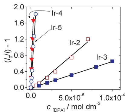
Fig. 21 Stern–Volmer plots generated from phosphorescence intensity quenching of complex Ir-2 ( \lambda_{\text{ex}} = 386 \text{ nm} ), Ir-3 ( \lambda_{\text{ex}} = 410 \text{ nm} ), Ir-4 ( \lambda_{\text{ex}} = 475 \text{ nm} ) and Ir-5 ( \lambda_{\text{ex}} = 425 \text{ nm} ). Phosphorescence was measured as a function of DPA concentration in \text{CH}_3\text{CN} . 1.0 \times 10^{-5} \text{ mol dm}^{-3} . 20^\circ\text{C} . Reproduced with permission from ref. 45b.
