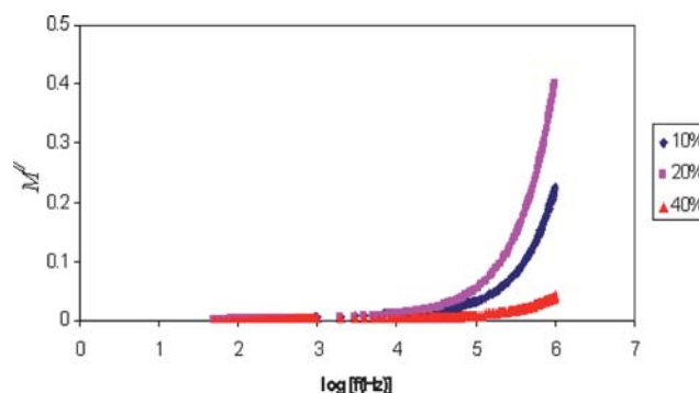
Fig. 6 Variation of the imaginary part of the modulus with frequency for PE-10, PE-20 and PE-40 samples.
