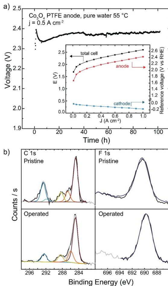
Figure 10. Long-term operation of a PTFE-containing anode. a) HEM electrolyzer operation with a \text{Co}_3\text{O}_4/\text{PTFE} -coated stainless-steel anode PTE, TP-85 membrane, and Pt-black TP-85 cathode for 100 h. Inset shows cathode and anode contributions to total cell voltage. b) XPS of the anode catalyst layer before and after 100 h operation.
