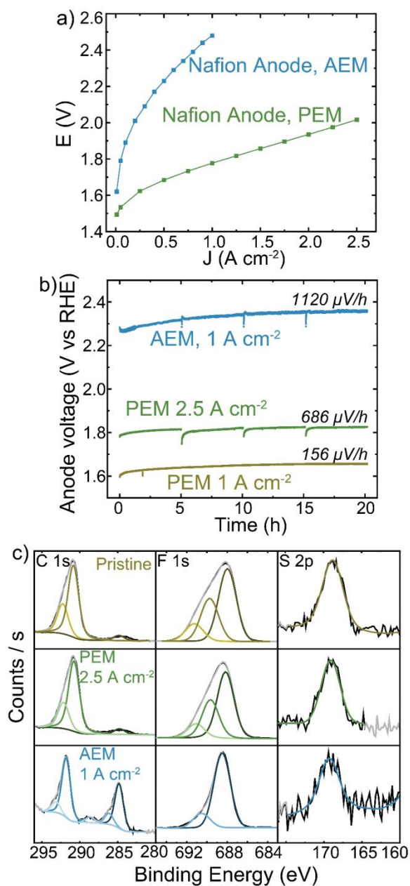
Figure 7. Nafion PTE operation in different membrane-pH environments. All cells were operated with a Nafion/ \text{IrO}_x catalyst on Pt/Ti anode, TP-85 or Nafion membrane, and Pt-black/TP-85 or Pt-black/Nafion cathode (matching the membrane). a) polarization comparison of Nafion PTE operating in a PEM MEA (green) and HEM MEA (blue). b) Nafion anode durability when operating in a PEM MEA at 1 \text{ A cm}^{-2} (yellow) and 2.5 \text{ A cm}^{-2} (green) and HEM MEA at 1 \text{ A cm}^{-2} (blue). c) XPS of Nafion PTEs before operation (yellow), after operation with a PEM MEA at 2.5 \text{ A cm}^{-2} (green) and after operation with a HEM MEA at 1 \text{ A cm}^{-2} (blue). Degradation at the Nafion anode PTE is only observed when operating with a HEM.
