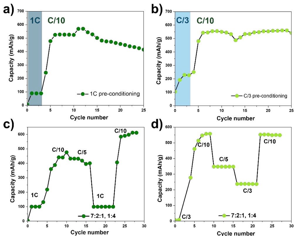
Figure 4: Fast Rate Preconditioning of Zn- \text{MnO}_2 Full Cells a) with 1C rate for three cycles and b) with C/3 rate for three cycles. c) and d) are rate tests at room temperature (RT), starting with 1C and C/3, respectively.
