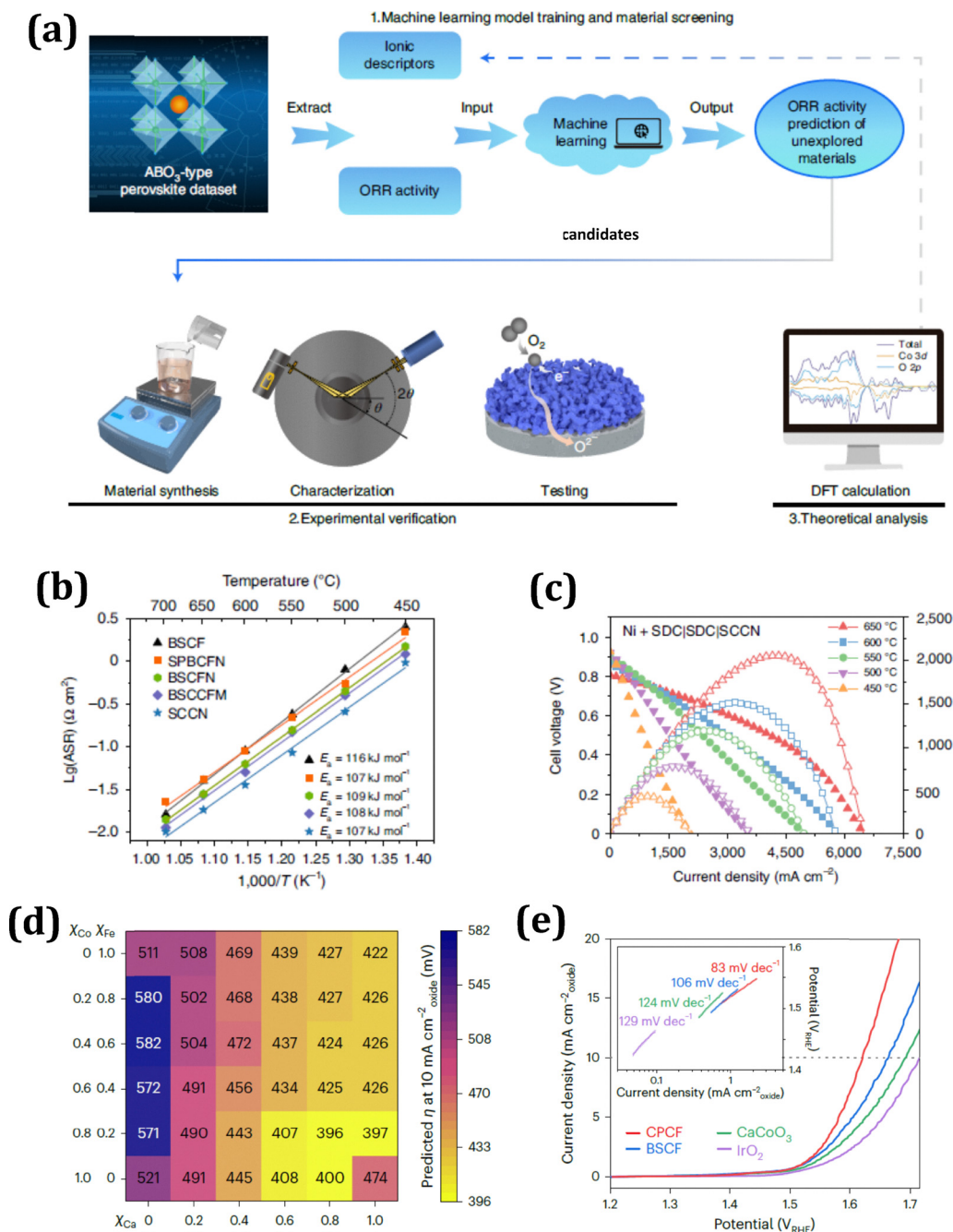
Fig. 8 (a) The overall workflow diagram: machine learning model training, material screening, experimental verification, and DFT analysis. \theta is X-ray incidence angle. (b) Arrhenius-type plots of ASR values of SCCN, BSCCFM, BSCFN, and SPBCFN. (c) Current density–voltage–power density curves of a single cell with the configuration Ni/SDC|SDC|SCCN at 450–650 °C. Reproduced with permission. 262 Copyright 2022, Nature. (d) The predicted overpotential at 10 \text{mA cm}^{-2} of \text{Ca}_x\text{Pr}_{1-x}\text{Co}_y\text{Fe}_{1-y}\text{O}_3 ( 0 \leq x, y \leq 1 ) oxides according to the precursor mixture ratio of Ca, Pr, Co and Fe. (e) Quantification of the electrochemical properties of CPCF compared to standard catalysts: linear sweep voltammetry curves. The inset shows Tafel slopes. Reproduced with permission. 263 Copyright 2023, Nature.
