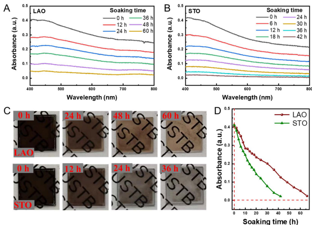
Fig. 4 Decomposition process of LCO thin films with 60 nm thickness soaked in 10% \text{CH}_3\text{COOH} solution. (A and B) Optical absorption spectra of LCO films on LAO (A) and STO (B) substrates at different times. (C) Optical photographs of LCO films on LAO and STO substrates ( 10 \times 10 \text{ mm}^2 ) at different times. (D) Curves of absorbance ( \lambda = 400 \text{ nm} ) variation of LCO films on the two substrates with soaking time.
