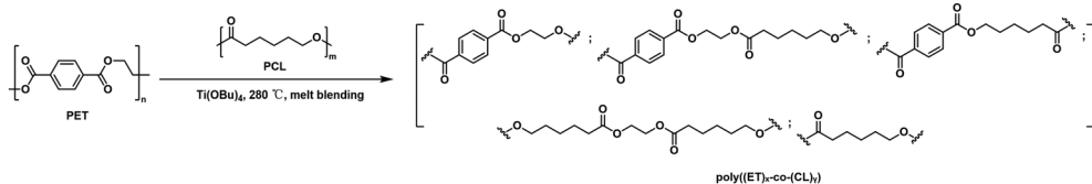
Fig. 10 Synthesis of \text{poly}((\text{ET})_x\text{-co-(CL)}_y) via transesterification of PET and PCL through melt blending.
