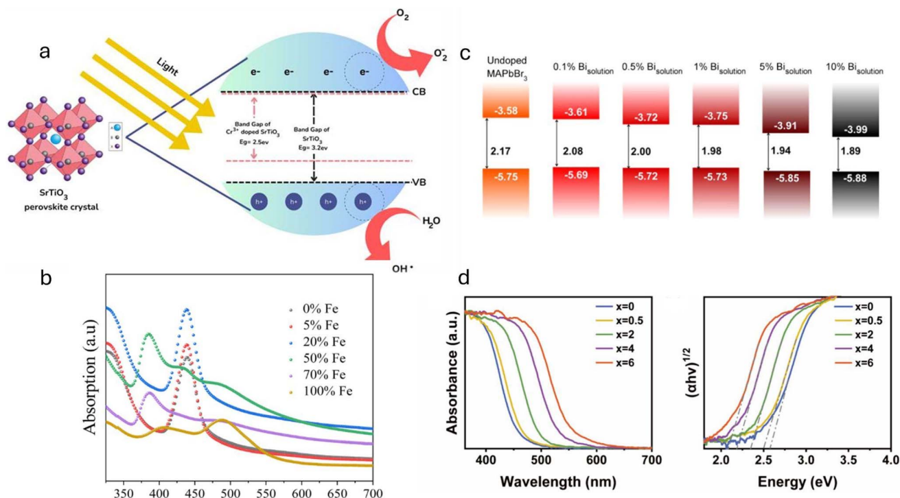
Fig. 5 Illustration of the effect of doping on the band structure and resulting optical properties in different perovskites. (a) A schematic diagram illustrating the electronic band structures for \text{SrTiO}_3 upon \text{Cr}^{3+} doping. Doping with \text{Cr}^{3+} introduces new electronic states within the bandgap, which can significantly improve its photocatalytic efficiency upon irradiation. (b) Variation in the bandgap alignment of \text{CH}_3\text{NH}_3\text{PbBr}_3 crystals with change in Bi% (Reproduced from ref. 93 with permission from American Chemical Society, Copyright 2016) (c) shift in the UV-vis absorption upon Fe incorporation in \text{Cs}_3\text{Bi}_2\text{Br}_9 (Reproduced from ref. 94 with permission from Royal Society of Chemistry, Copyright 2024). (d) UV-vis absorption spectra and corresponding Tauc plots of \text{Cs}_2\text{AgBiCl}_{6-x}\text{Br}_x with varying concentration of Br (Reproduced from ref. 95 with permission from American Chemical Society, Copyright 2025).
