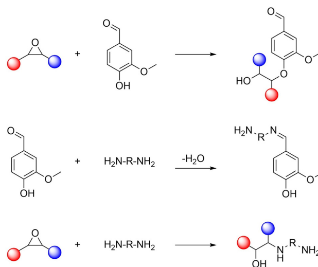
Fig. 11 Reactions involved in vanillin-based vitrimers based on imine–imine and amine–imine exchange reactions. Adapted from ref. 79 with permission from American Chemical Society, Copyright © 2024.
