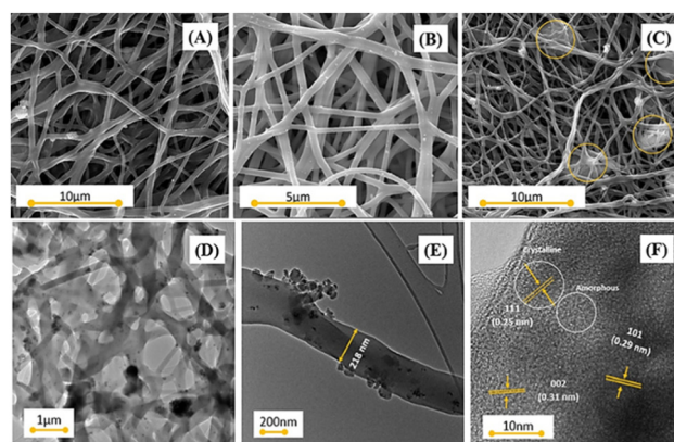
Fig. 2 SEM images of (A) 20 wt%, (B) 40 wt%, and (C) 60 wt% samples. (D) TEM images of the 40 wt% sample, (E) the size of the fiber and (F) different crystalline planes of CuO–ZrO 2 NPs in the amorphous PAN matrix.
