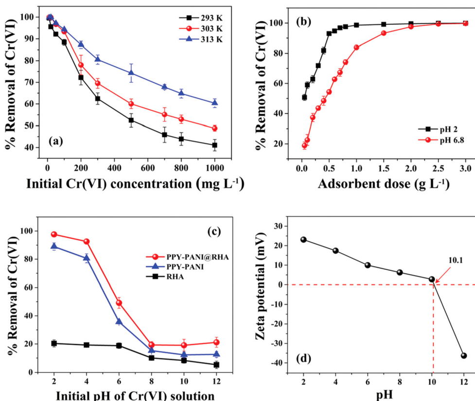
Fig. 25 (a) Effect of initial concentration of Cr(VI) at a different temperature (PPY PANI@RHA dose: 0.8 g L -1 ; contact time: 300 min; agitation speed: 200 rpm; pH ~2), (b) effect of adsorbent dose at pH 2 and without pH (~6.8) adjustment (initial Cr(VI) concentration: 50 mg L -1 ; contact time: 300 min; agitation speed: 200 rpm; temperature: 303 K), (c) effect of initial solution pH on % removal of Cr(VI) by PPy–PANI@RHA, PPy–PANI and RHA adsorbents (Initial Cr(VI) concentration: 50 mg L -1 ; contact time: 300 min; agitation speed: 200 rpm; temperature: 303 K), and (d) variation of zeta potential of PPy–PANI@RHA at different pH. 448 Reproduced with permission from RSC.
