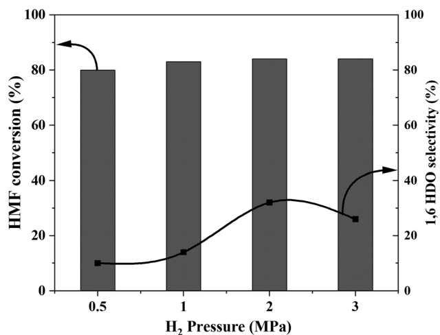
Fig. 6 Effect of the hydrogen pressure during the ring opening hydrogenolysis of HMF over 5% RuPt/HAP. Reaction conditions: HMF: 1.59 mmol; methanol: 20 mL; temperature: 120 °C; time: 5 h; HMF/total metal molar ratio: 155.
