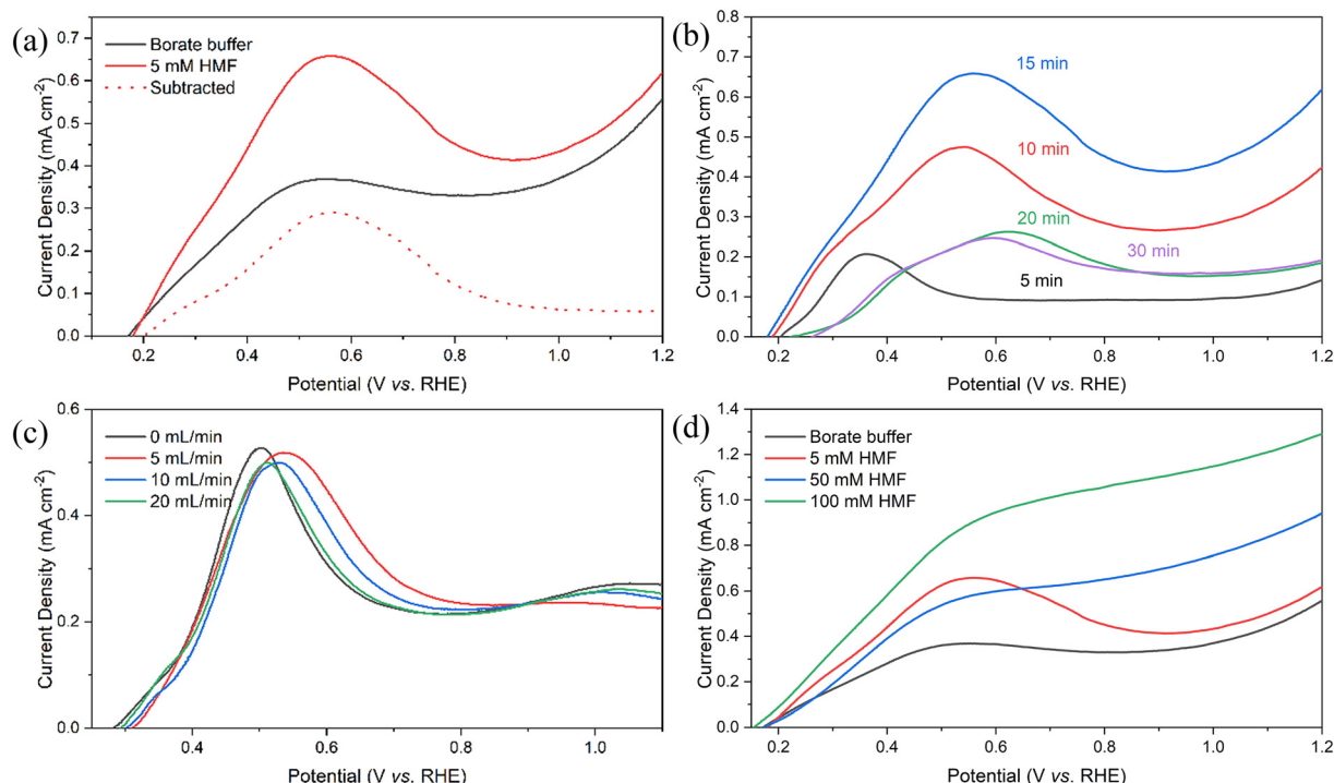
Fig. 9 Photocurrent response of \text{Ni(OH)}_2 -decorated \text{BiVO}_4 photoanodes under AM 1.5 G illumination ( 100 \text{ mW cm}^{-2} ). (a) LSV scans of a 15 minute electrodeposited electrode measured in borate buffer with (red) and without (black) 5 mM HMF. The dotted line represents the net photocurrent obtained by subtracting the baseline response in buffer alone. (b) LSV scans of \text{BiVO}_4 electrodes electrodeposited with \text{Ni(OH)}_2 for various deposition times from 5 to 30 minutes, measured in borate buffer with 5 mM HMF. (c) LSV scans in 5 mM HMF measured at different electrolyte flow rates using a laminar flow cell. (d) LSV responses recorded with varying HMF concentrations in a batch reactor with agitation. Scan rate = 10 \text{ mV s}^{-1} .
