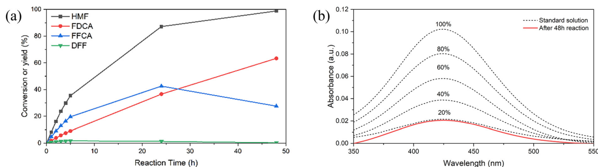
Fig. 4 Product analyses of a 48 hour TEMPO-mediated PEC reaction. (a) HMF conversion (started with 5 mM) and yields of the oxidation products. (b) Normalised UV-vis spectrum of post-reaction electrolyte compared to standard TEMPO solutions (100% represents 7.5 mM at the start of the reaction).
