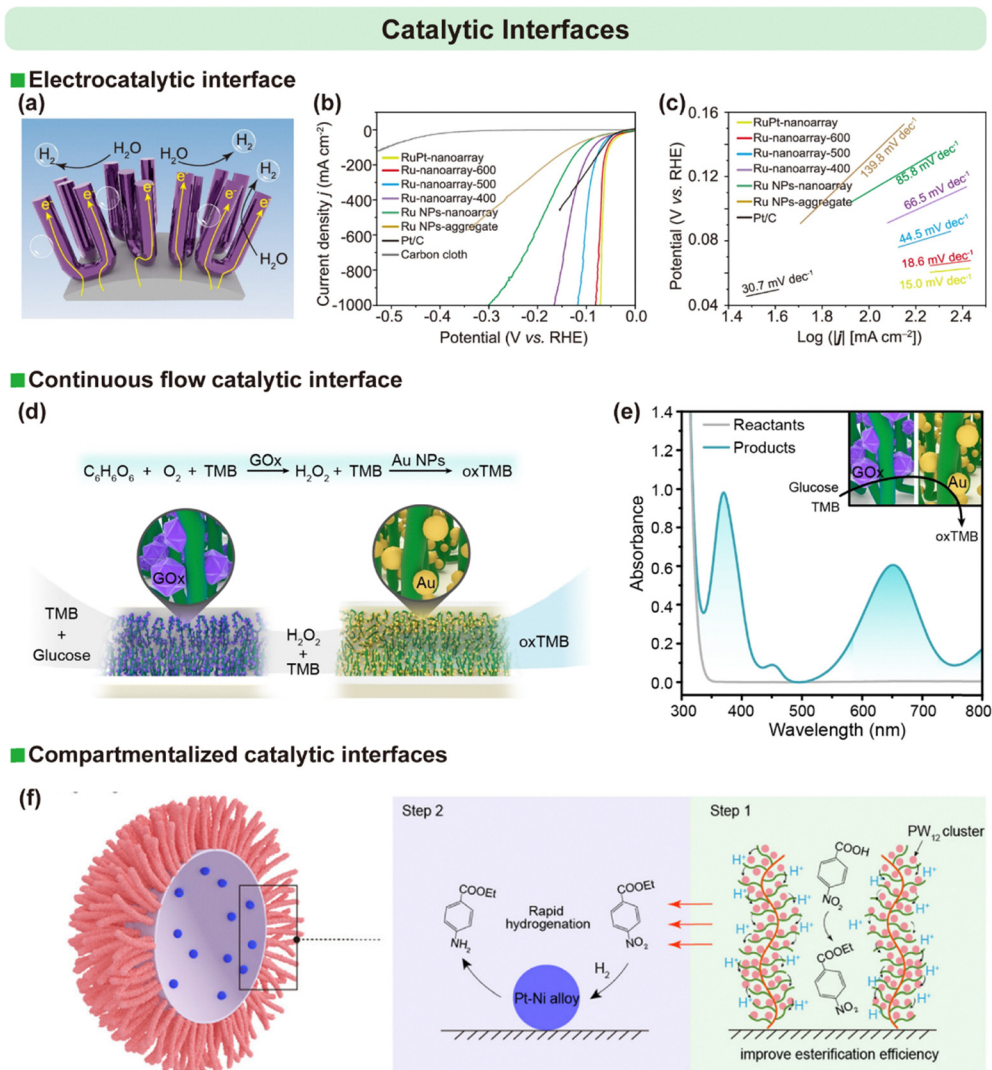
Fig. 17 (a) Schematic representation of a metallic Ru nanoarray designed for the hydrogen evolution reaction (HER). (b) iR-corrected polarization curves in 0.5 M H 2 SO 4 solution for alloy RuPt nanoarray, metallic Ru nanoarray- T , Ru NP nanoarray, Ru NP aggregates, commercial Pt/C-decorated carbon cloth, and pristine carbon cloth. (c) Tafel plots derived from the polarization curves shown in (b). Reproduced from ref. 54 with permission from Springer Nature, Copyright 2025. (d) and (e) Illustration and UV-vis spectra for a cascade reaction in PBS (pH 5.05) sequentially catalyzed by GOx-functionalized micellar brushes and Au NP-functionalized micellar brushes. Reproduced from ref. 51 with permission from Wiley, copyright 2021. (f) Schematic diagram of the sequential tandem conversion of p -nitrobenzoic acid within a microreactor engineered via surface modification strategies. Reproduced from ref. 55 with permission from Wiley, copyright 2025.
