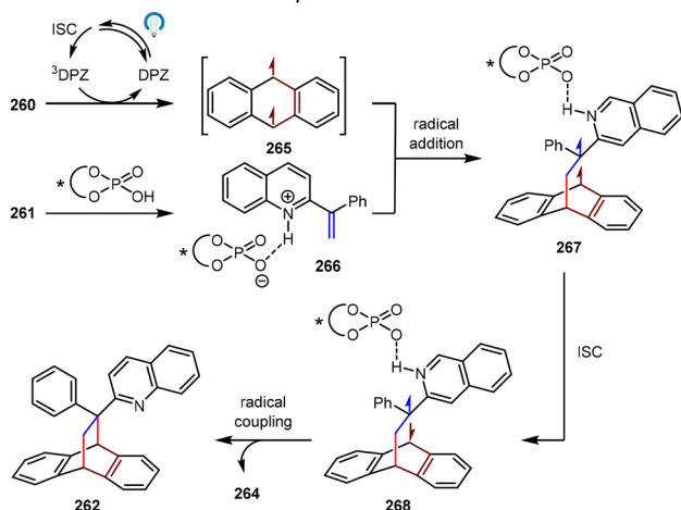
Scheme 53 Asymmetric [4+2] dearomatic photocycloadditions of anthracene with alkenylazaarenes.
