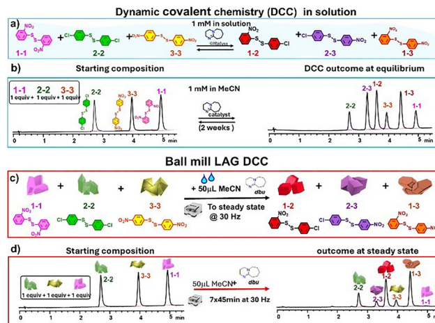
Fig. 15 Outcome of disulfide exchange among three equimolar homodimers (1-1, 2-2, 3-3) in the presence of DBU leading to the formation of 3 heterodimers 1-2, 2-3, 1-3. (a) and (b) Solution DCC (1 mM, MeCN) of three equimolar homodimers (1-1, 2-2, 3-3) in the presence of DBU; (a) reaction scheme; (b) outcome of solution DCC at steady-state monitored by HPLC. (c) and (d) Ball mill LAG (MeCN) of three equimolar homodimers (1-1, 2-2, 3-3) in the presence of DBU. (c) Reaction scheme; (d) outcome of ball mill LAG milled to steady-state and monitored by HPLC. 41 Adapted from ref. 41 with permission from The Royal Society of Chemistry.
